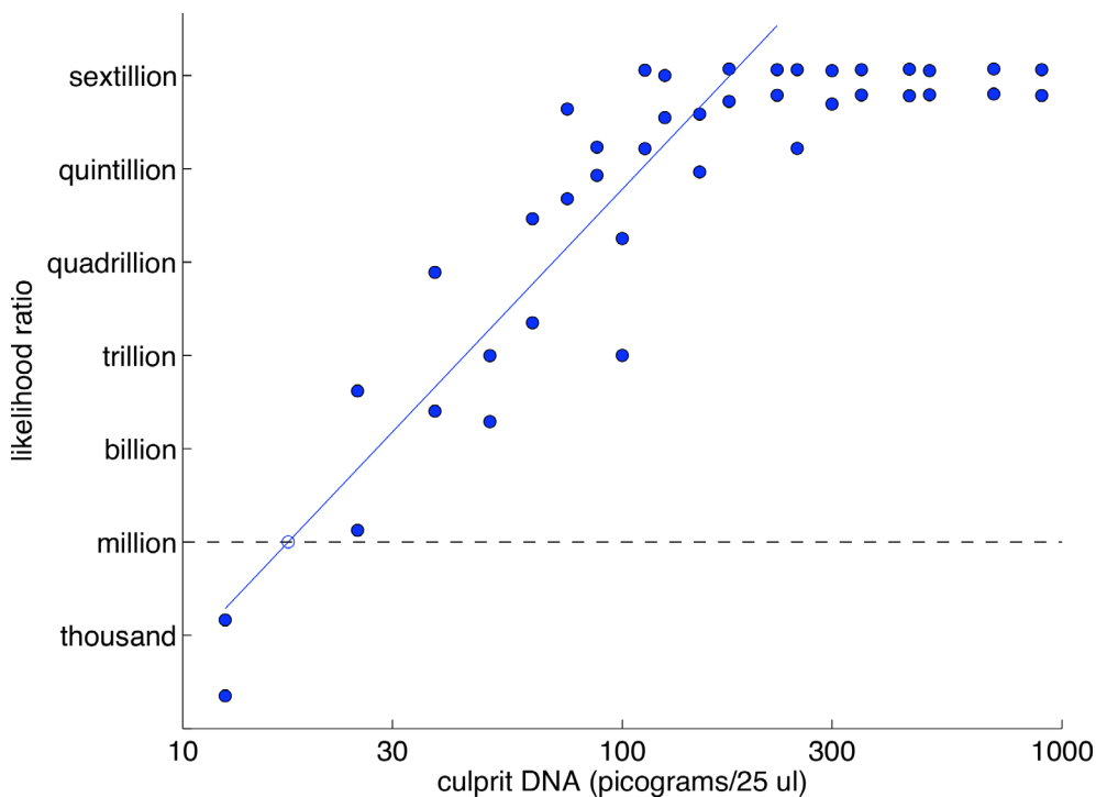
FIG. 1—Linearity. Scatterplot showing \log(LR) match information (y-axis) versus \log(DNA) (x-axis) for TrueAllele analysis of forty two-person mixtures solved assuming a known contributor genotype. The data (blue dots) follow an increasing regression line ramp (solid blue line) that plateaus once reaching maximum match information. The million LR match level is shown (dashed gray line). Reproduced from (20) with permission of the author ( https://doi.org/10.1371/journal.pone.0008327.g007 ). [Color figure can be viewed at wileyonlinelibrary.com ]
