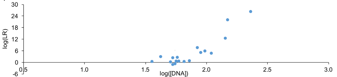
FIG. 5—DNA amount. Plots show how match statistics depend on DNA amount for different numbers of contributors. The horizontal axis gives the logarithm of DNA contributor amount (picograms). The vertical axis shows log(LR) match statistics. The plots are shown for (a) two through (e) six observed unknown contributors. [Color figure can be viewed at wileyonlinelibrary.com]
